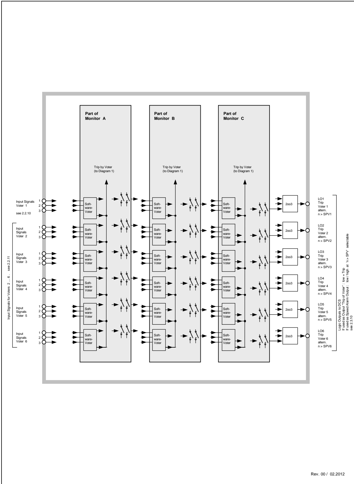
Figure 3: E16x446 System Structure Diagram 2 of 2
