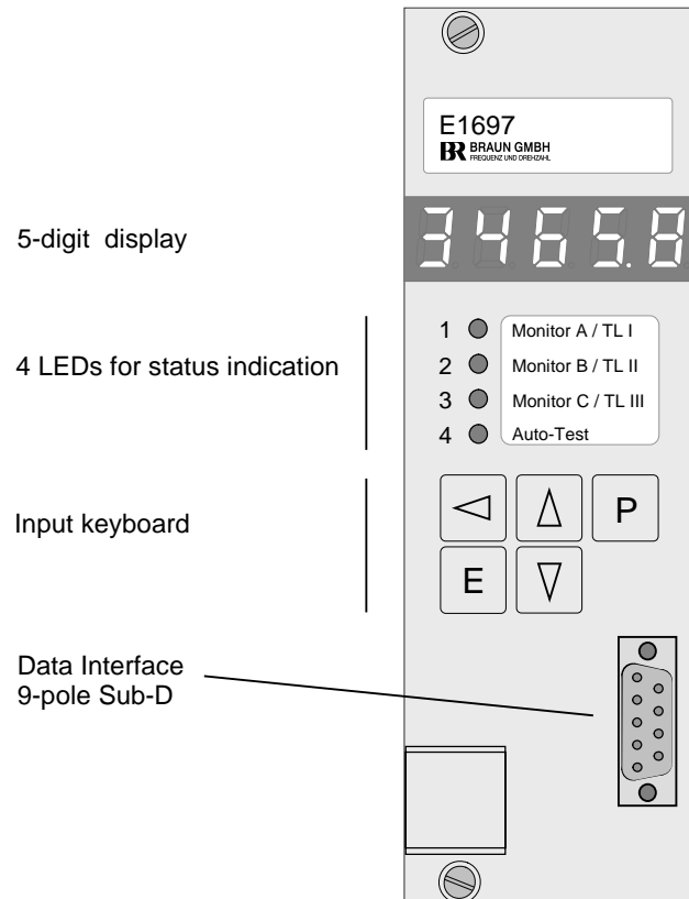
Figure 11: Front view of Test-Generator E1697
