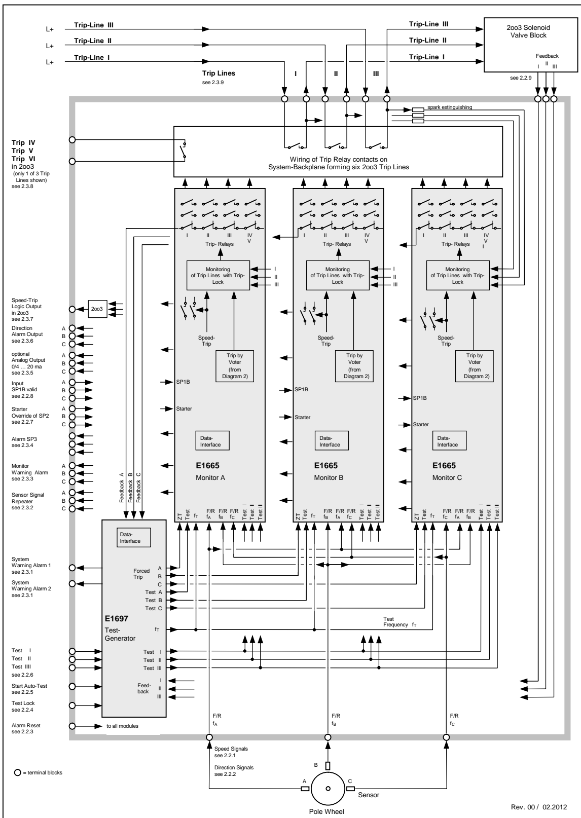
Figure 2: E16x446 System Structure Diagram 1 of 2
