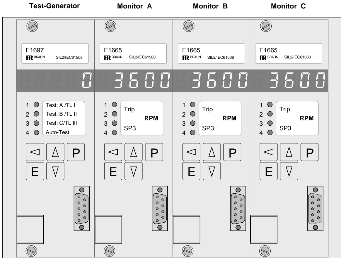
Figure 1: E16x446 System Front View
