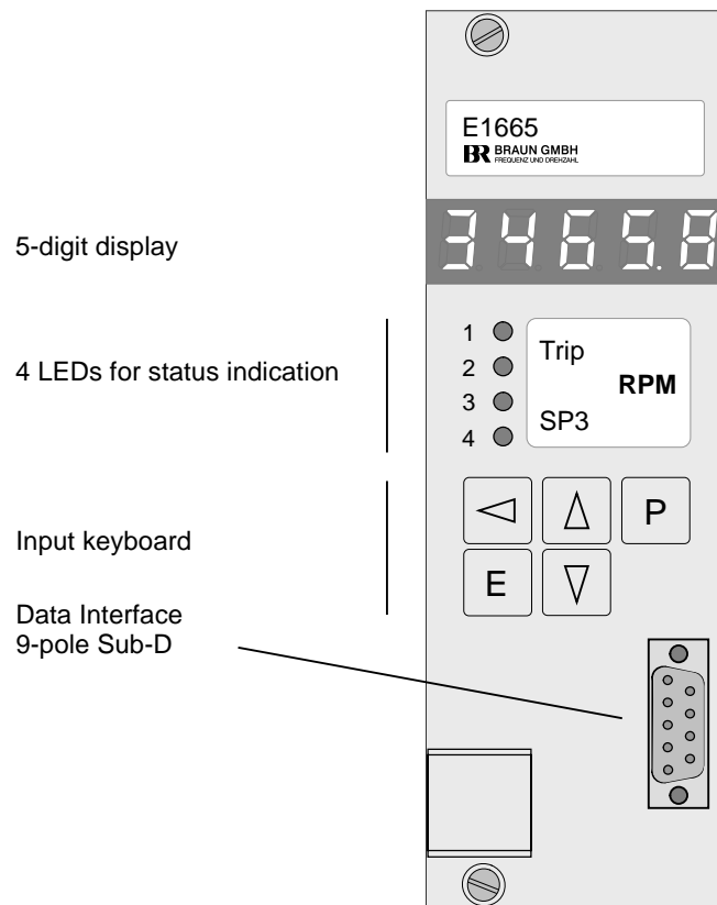
Figure 10: Front view of Monitor E1665
