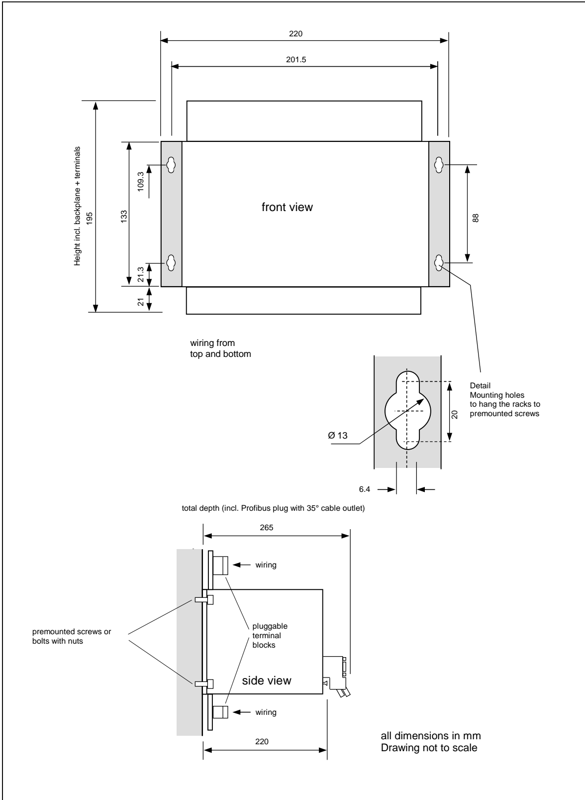
Figure 7: Dimensions of System E16A446
