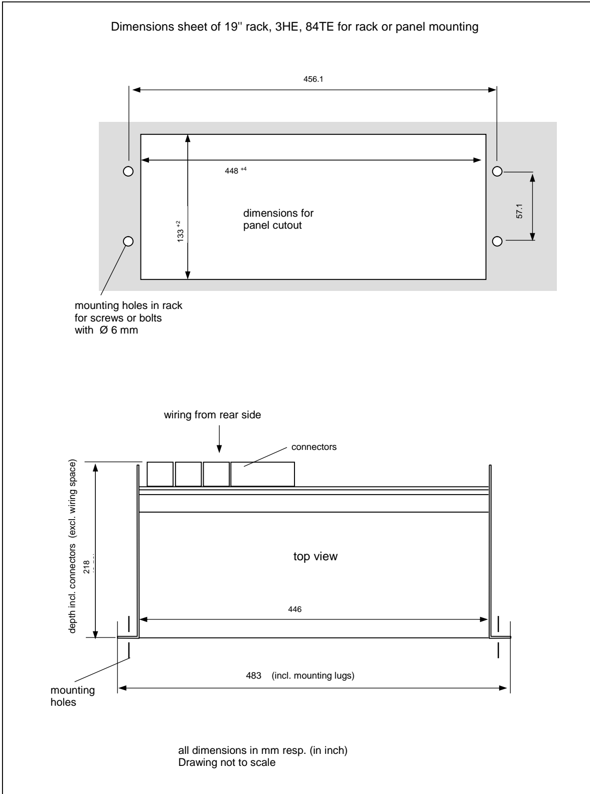
Figure 8: Dimensions of System E16E446
